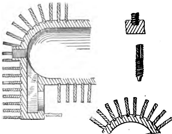
FIG. 297.—The "Knox" Pin-Cooled Cylinder. In this engine, pins are used for radiating instead of the usual flanges or ribs as on other air-cooled cylinders.
